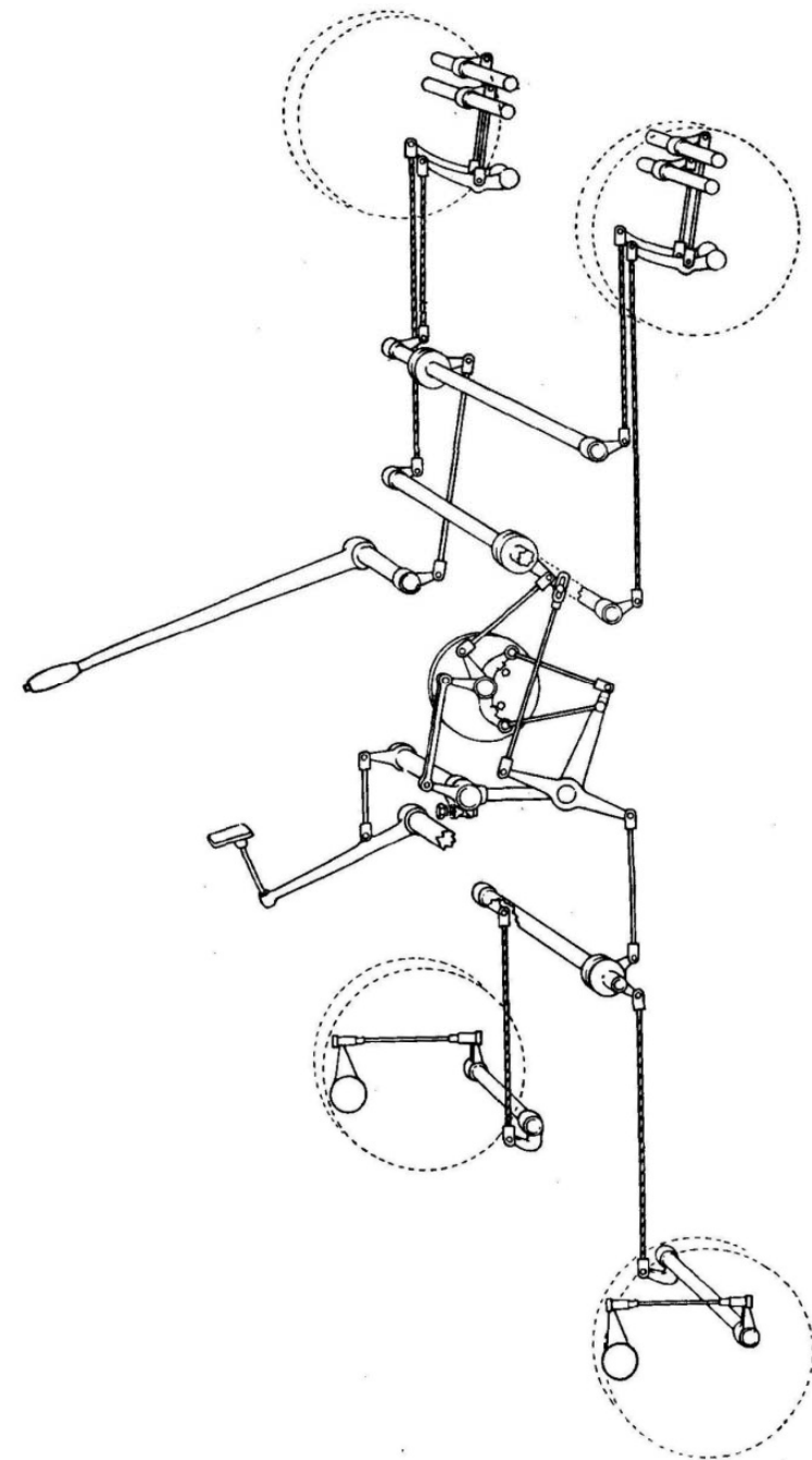
DIAGRAM OF ROLLS-ROYCE FOUR-WHEEL BRAKE SYSTEM.
